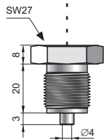
G1/2 type M type G1/2", Ø4 hole M20x1.5, Ø4 hole
