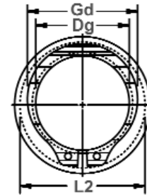
Clearance Diameter & Gaging Diameter
