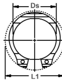
Clearance Diameter & Gaging Diameter
