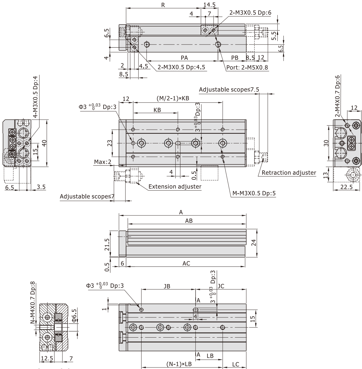
Across A-A
