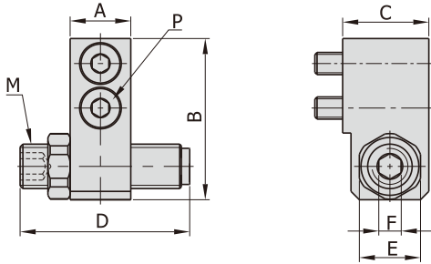
Body Mounting
