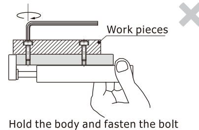
Hold the body and fasten the bolt
