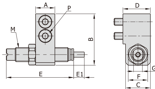
Body Mounting
