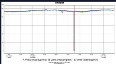
Voltage Trends
