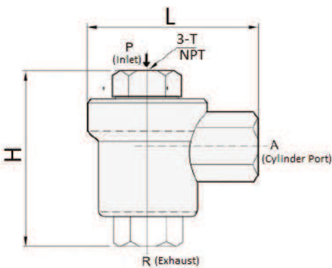
Dimensions (mm)
