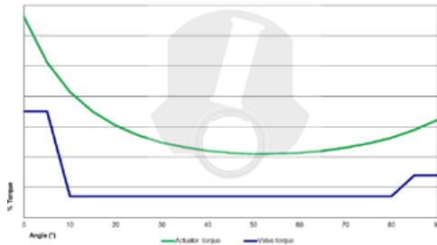
DOUBLE ACTING - CANTED YOKE
