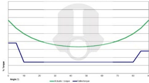
DOUBLE ACTING - SYMMETRIC YOKE
